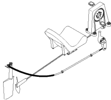
Steering and drive system
