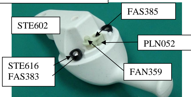
Back side of steering handle
