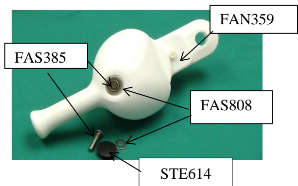
Front side of steering handle
