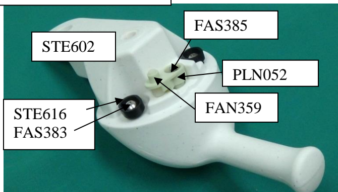
Back side of steering handle
